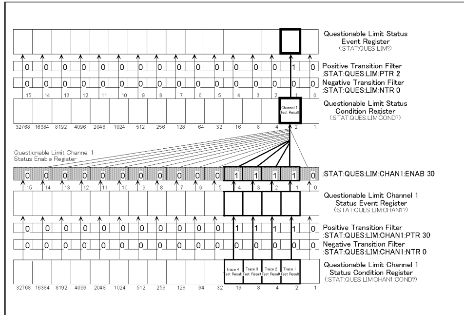
Obtaining the test results for a channel (channel 1 in this example) using the status register
